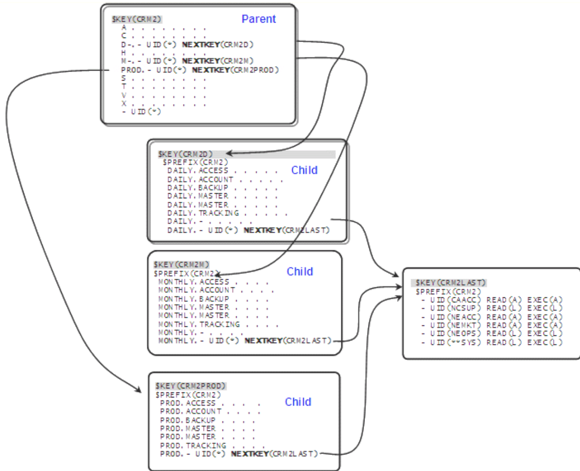
Figure 65. Rule structure
